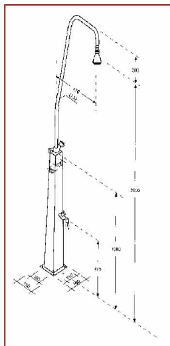
620006 Infinity 1 plus Mixing battery with drain cock
