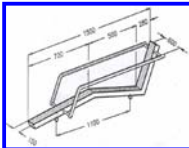
740120 Single bed complete with handrail
