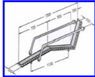
740122 Single bed complete with handrail for liner
