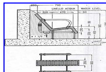
740125 Single arm-chair complete with handrail for liner
